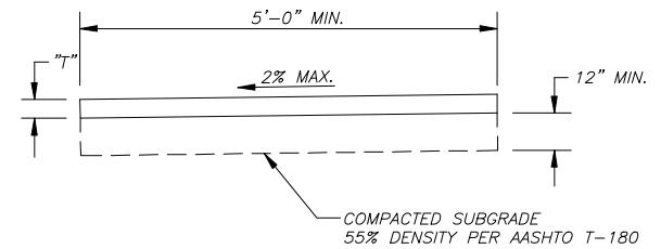
SECTION A-A CONCRETE TO BE CLASS I, 3000 psi
